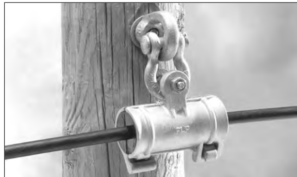
Anchor Shackle w/Eye Nut Option
